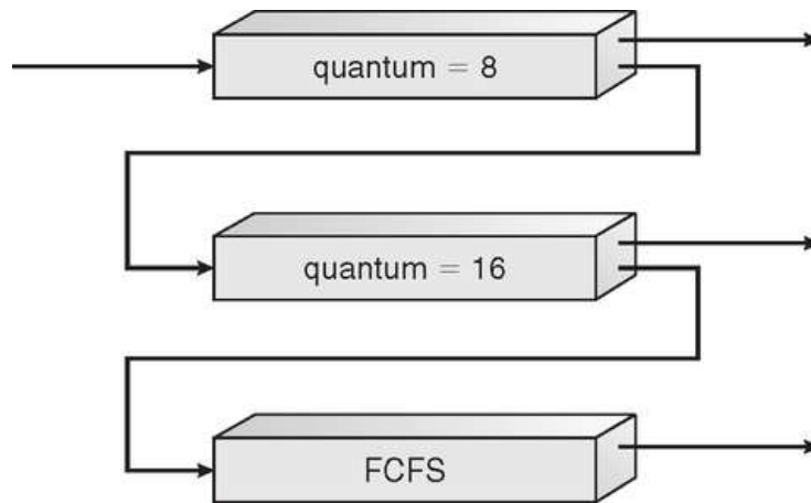
FIGURA 5.7 Multilevel feedback queues.
