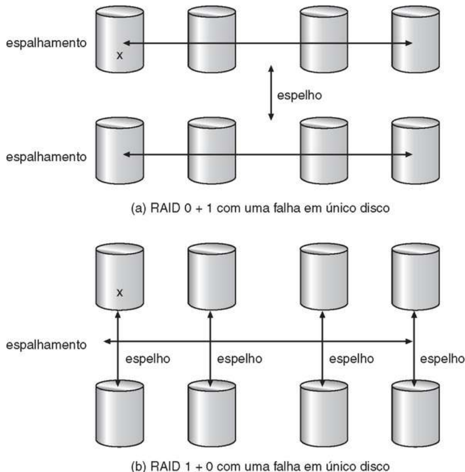
FIGURA 12.12 RAID 0 + 1 e 1 + 0.
