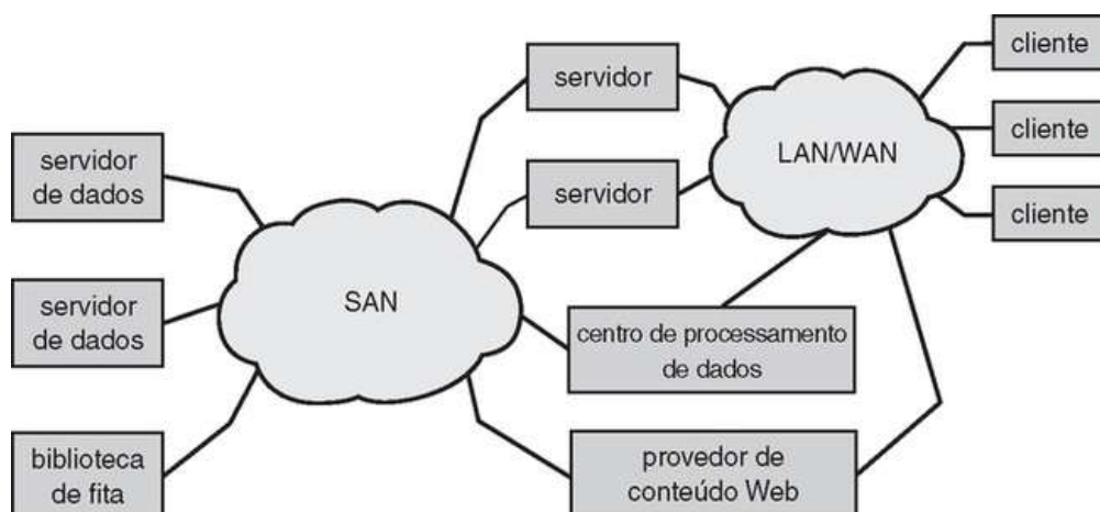
FIGURA 12.3 Storage-Area Network.
